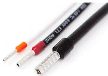
MKPW-10S 圧着形状
